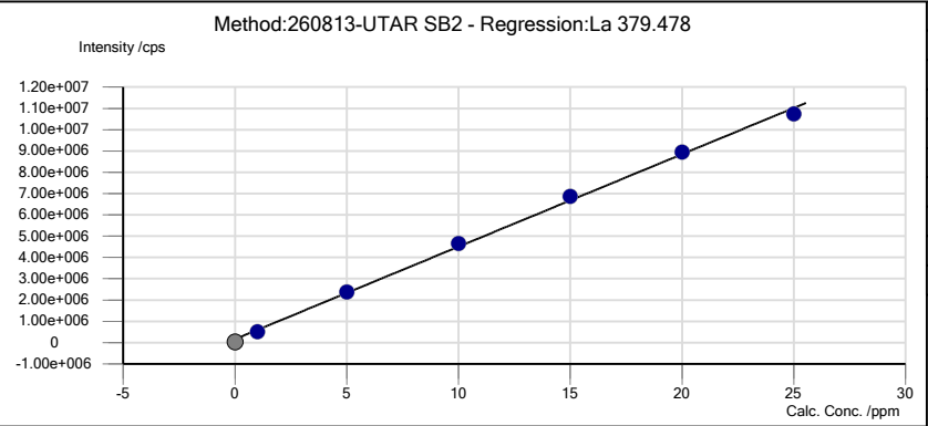
Regression Graph of La 379.478
