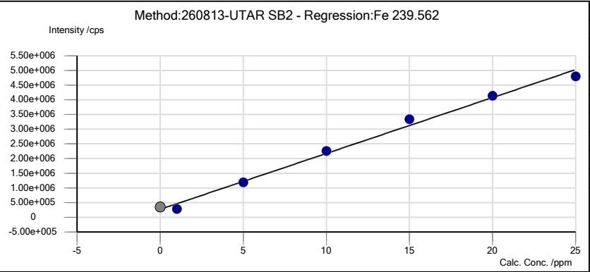
Regression Graph of Fe 239.562
