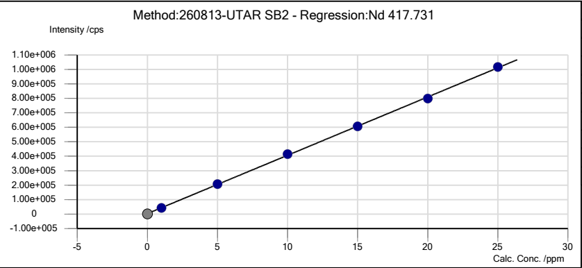
Regression Graph of Nd 417.731
