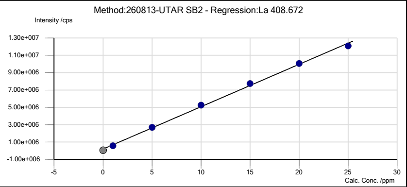
Regression Graph of La 408.672
