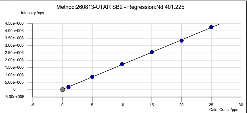
Regression Graph of Nd 401.225
