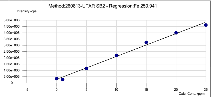
Regression Graph of Fe 259.941
