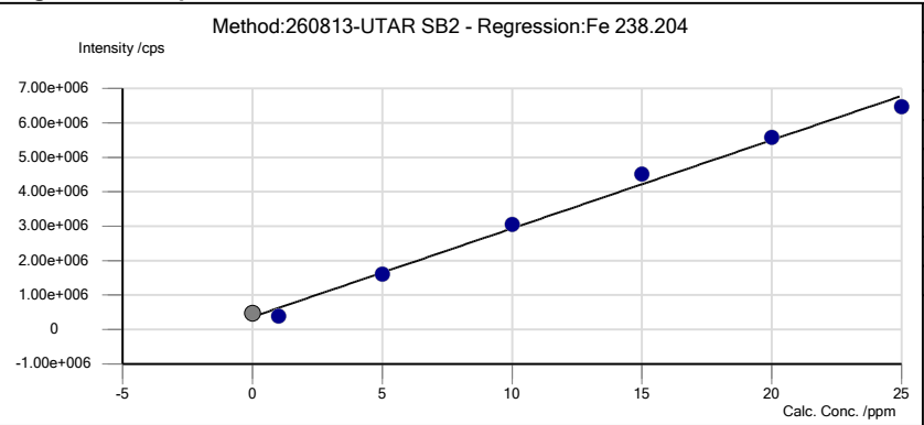
Regression Graph of Fe 238.204
